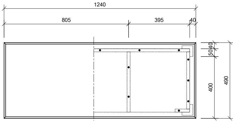
TOP SCALE 1:10
