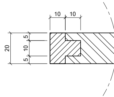
DETAIL 1:5
