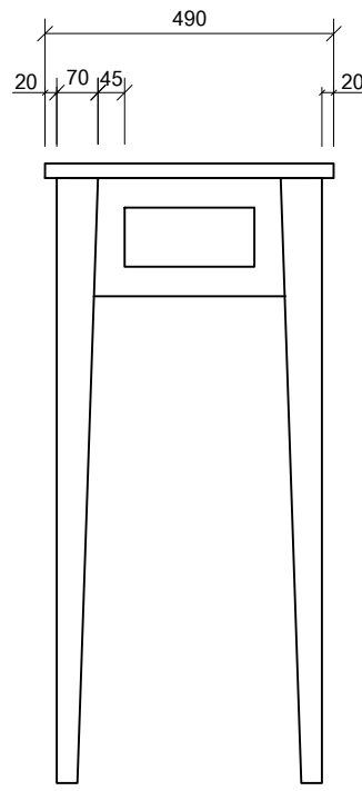
SIDE SCALE 1:10
