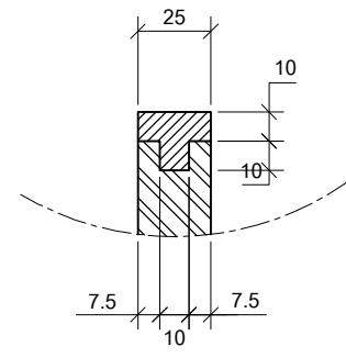
DETAIL 1:5
