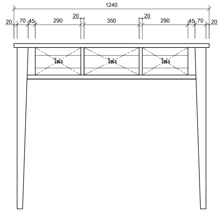
BACK SCALE 1:10
