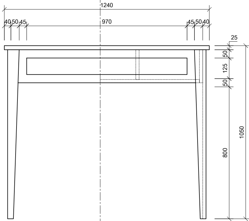
FRONT SCALE 1:10
